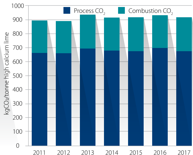
Emissions of CO 2 per tonne of standard purity high calcium lime
