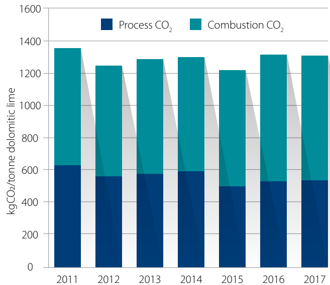
Emissions of CO 2 per tonne of dolomitic lime
