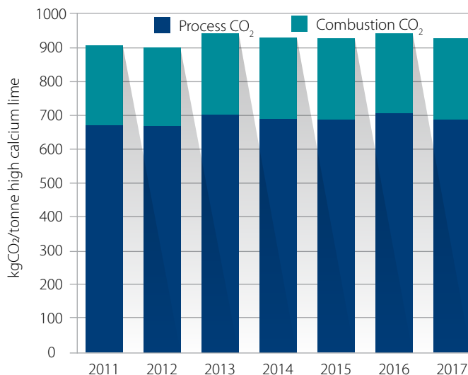
Emissions of CO 2 per tonne of high calcium lime
